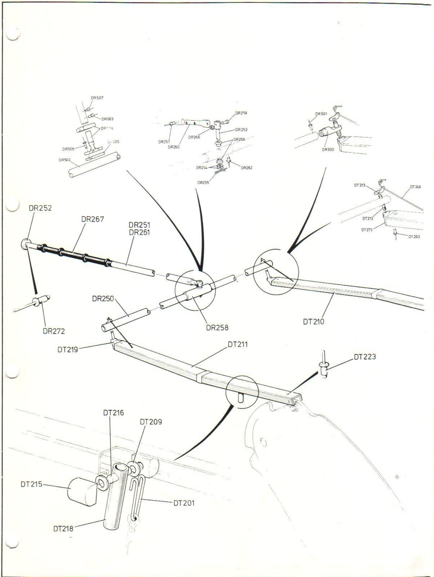
DRAWING 4 Rudder details
