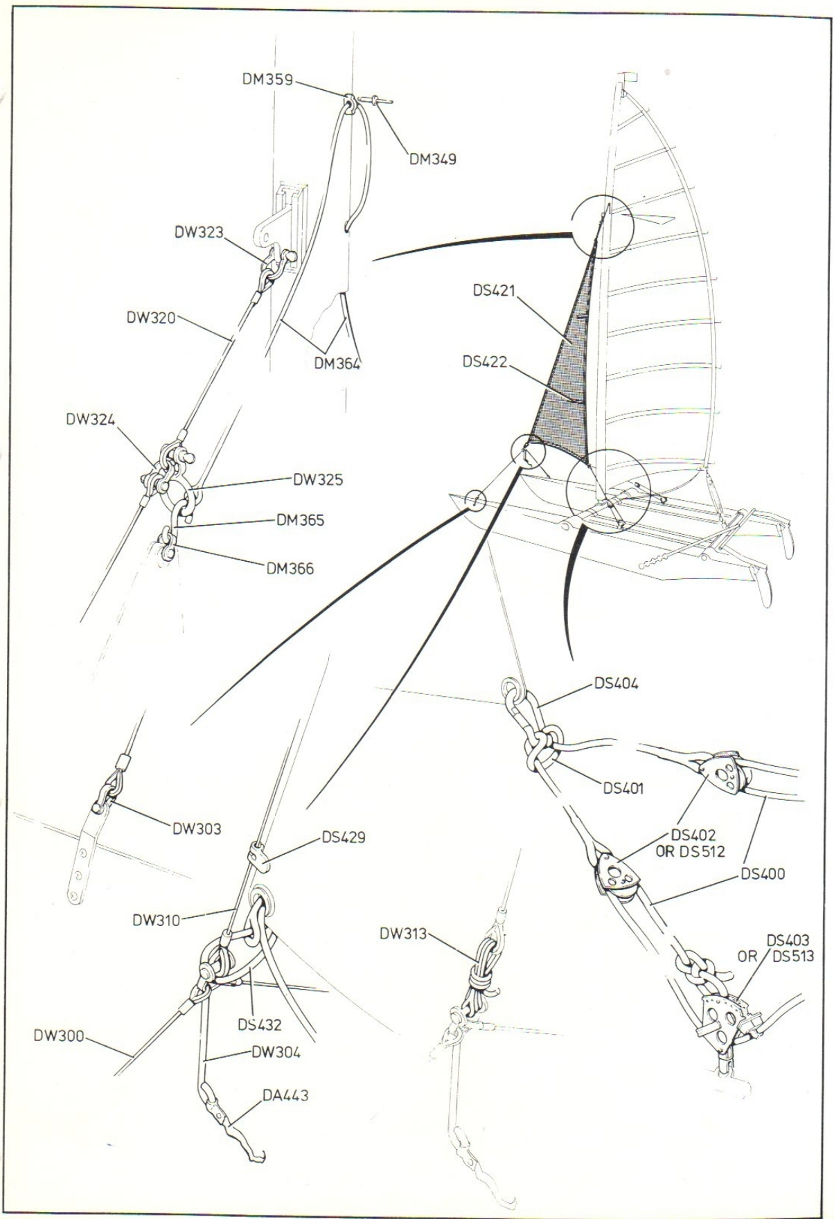
DRAWING 5 Jib details
